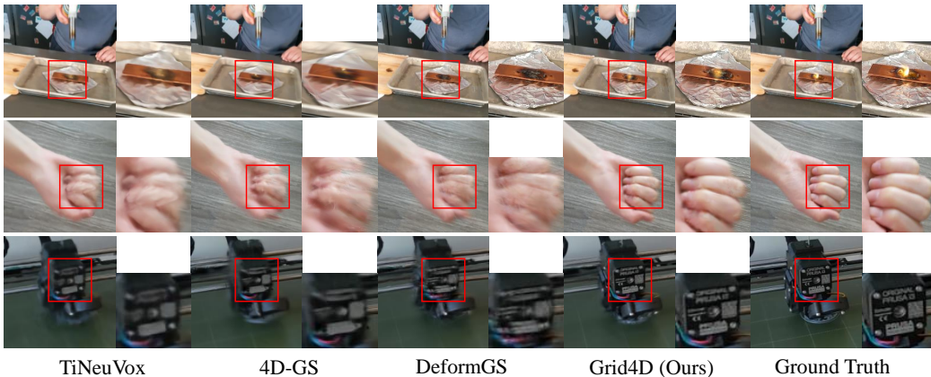
Figure 5: Qualitative comparisons on the real-world HyperNeRF [27] dataset.
