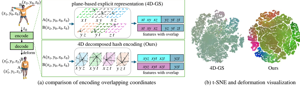
Figure 2: Comparison of our proposed 4D decomposed hash encoding with the plane-based explicit representation [43]. (a) Compared to the plane-based methods based on the low-rank assumption, our methods reduce the overlap ratio in the features from a half to a quarter when encoding points A and B with heavily overlapping coordinates. (b) is the t-SNE [38] visualization of all the features, and the colors denote the corresponding represented deformations. The diversity of colors demonstrates that the reduced overlap makes the features represent different deformations more effectively.
